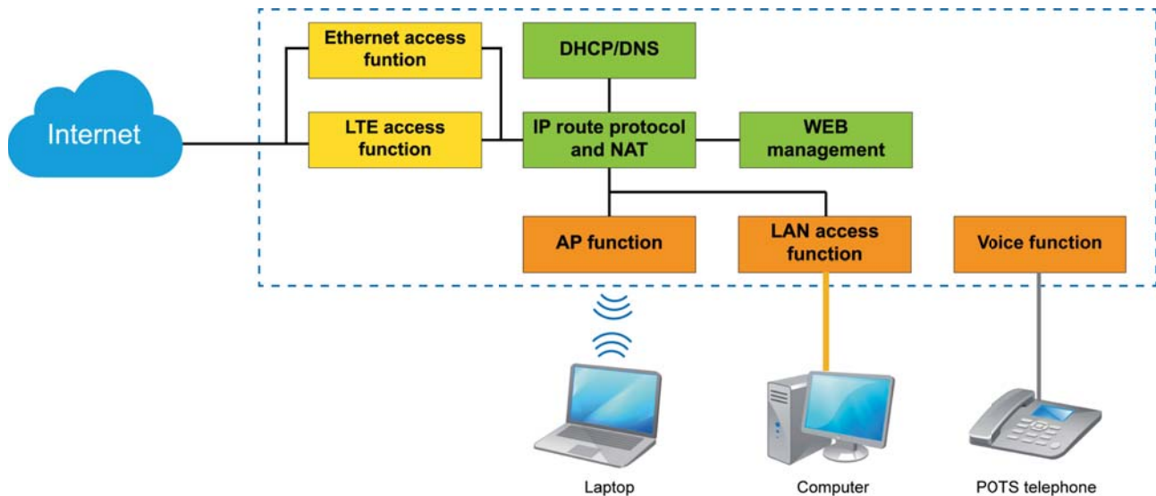
Figure 5-1 System architecture
